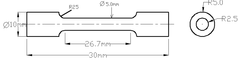
Fig. 1. Tensile Strength Test specimen
